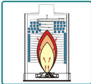
Schedule 80 pipe Heating coil, elliptically wound and stretched, no seam welds
